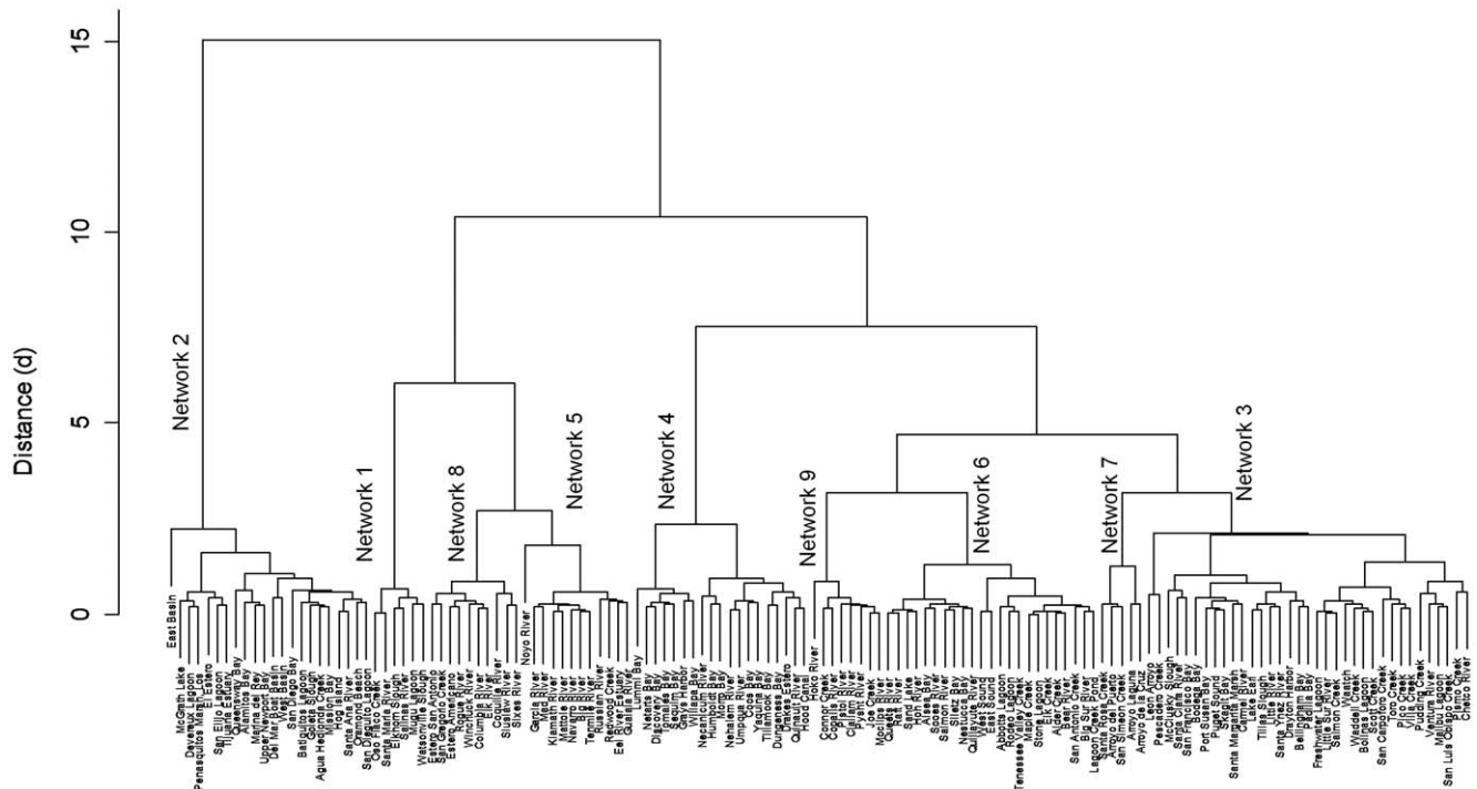
Figure 4. Dendrogram showing hierarchical division of estuary networks and agglomeration schedule. The hierarchical clustering identified nine substantive networks at a Euclidean distance of 2.5. Major divisions are by development (Network 2; d = 16 ), impaired inflows (Networks 1, 5, 8; d = 10 ), and approved shellfish growing areas (Networks 4; d = 7.5 ). doi:10.1371/journal.pone.0017407.g004
